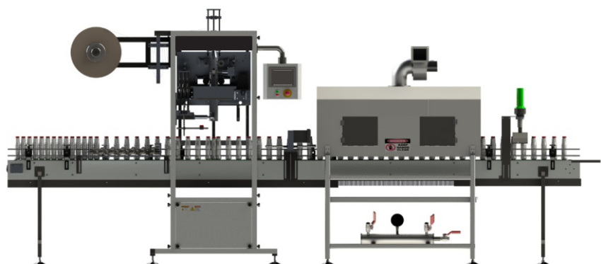
Sleeve Applicator
